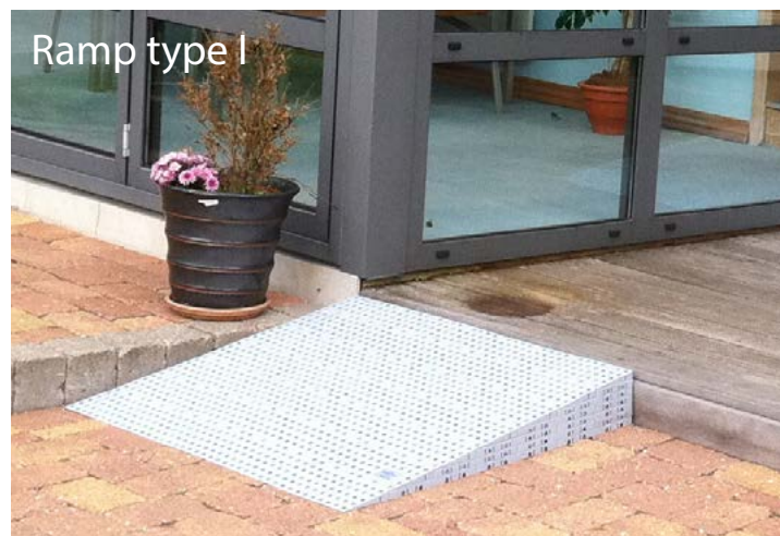
Ramp type I Inclination 1:7 Flat surface, great for electric wheelchairs.
