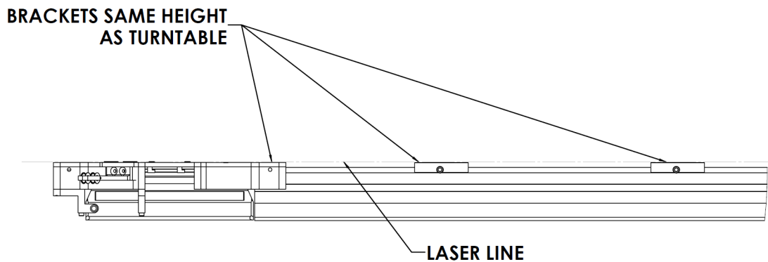
Figure 108: Install the Remaining Ceiling Track Brackets and Ceiling Track for the System at the Same Height as the Turntable
