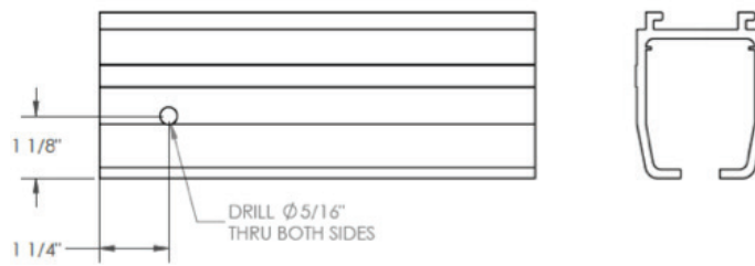
Figure 18: Clevis Pin Hole Location
