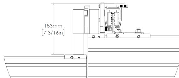
Figure 79: Track Plus System Bracket Height Difference—7 3/16"
