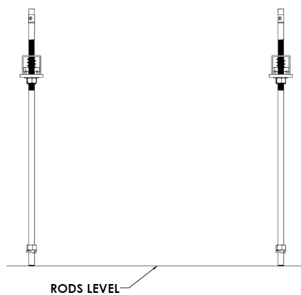
Figure 255: Bottoms of All Threaded Rods Level to Each Other
