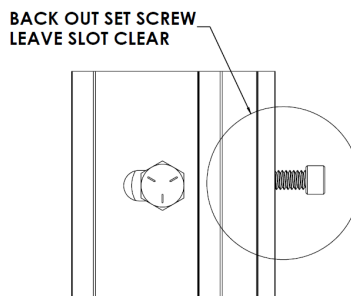
Figure 301: Loosen the Ceiling Bracket Set Screw So No Threads are Visible in the Bracket Channel
