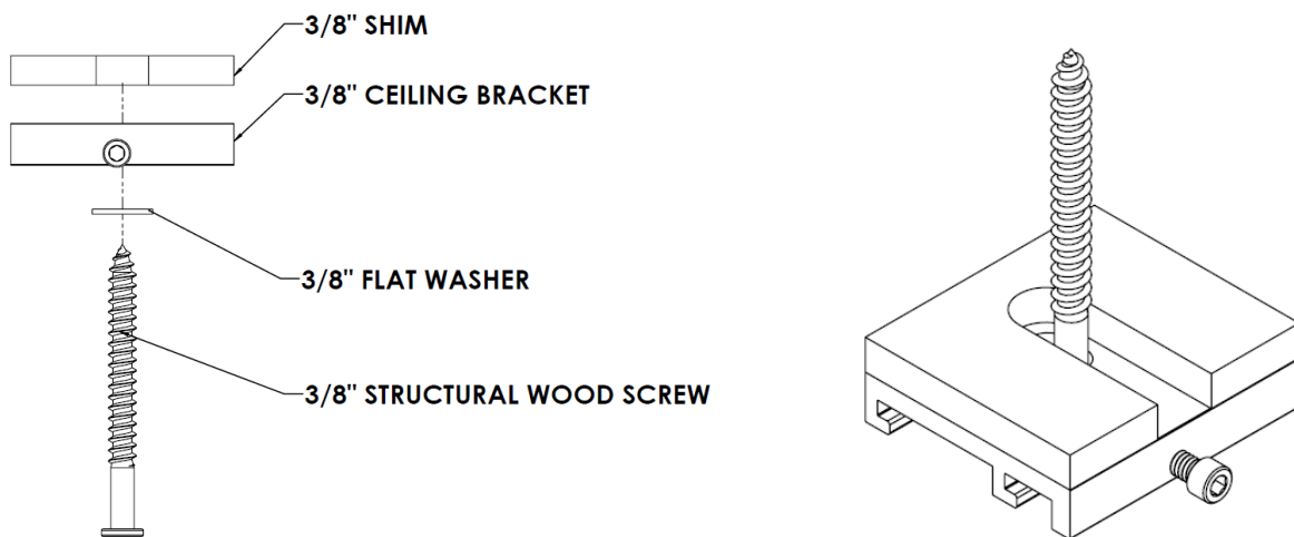
Figure 162: Wood Framing Bottom-Up Installation, Standard Mount—Structural Wood Screws and Joists (Detail)
