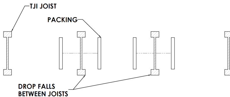
Figure 189: Ceiling Bracket Attachment Locations
