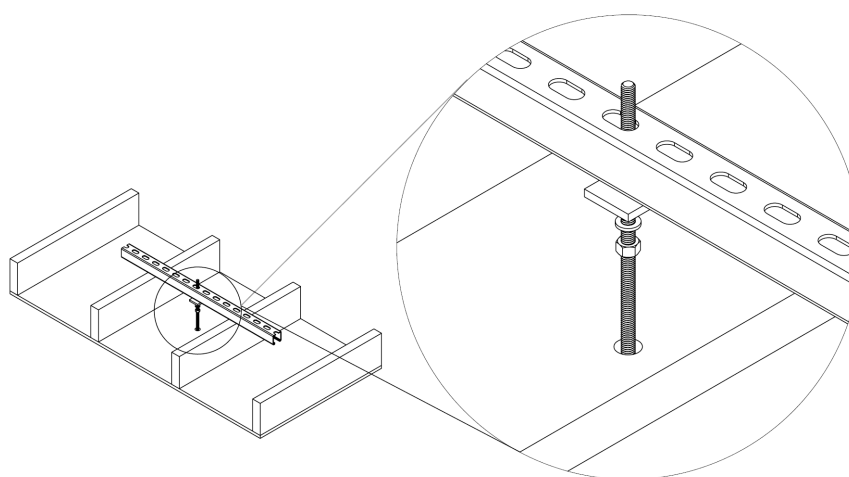
Figure 140: Threaded Rod Through Strut Slot
