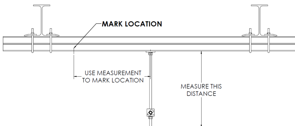
Figure 291: Perpendicular Brace
