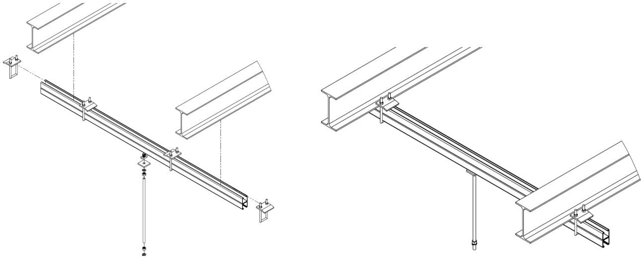
Figure 276: Structural Beam Attachment
