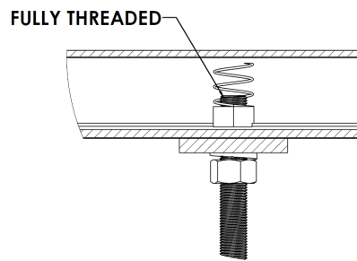
Figure 283: Threaded Rod Fully Threaded into the Strut Channel Nut
