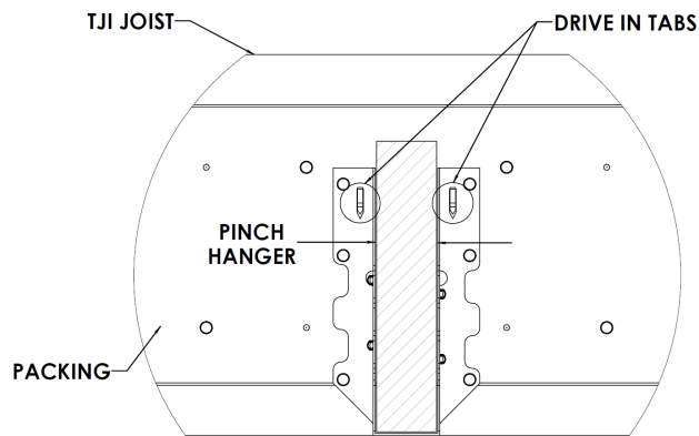
Figure 196: Joist Hanger Metal Tabs Hammered into the Packing
