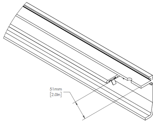
Figure 310: Measure from the Flush End of the Male Terminal Tabs the Length of the Track, Minus 4"
