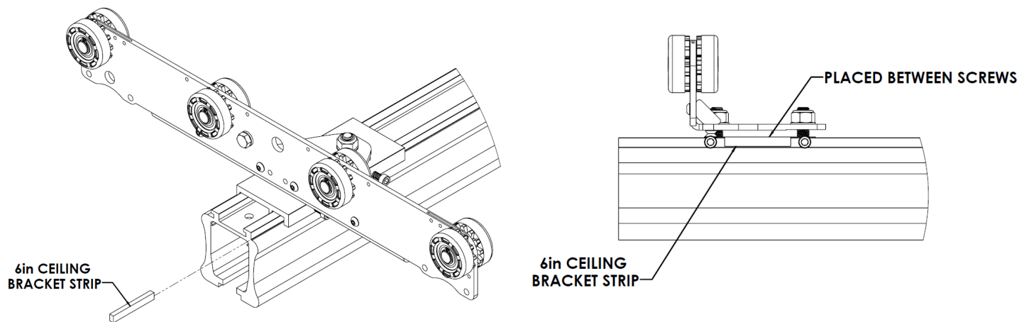
Figure 23: Bracket Strip Installation
