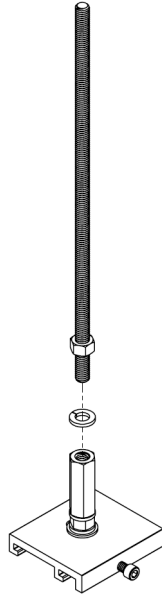
Figure 305: Level by Threading the 1/2" Coupling Nut Further On or Off of the Threaded Rod
