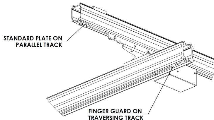
Figure 53: Exchange the Finger Guard with the Track Endstop Plate
