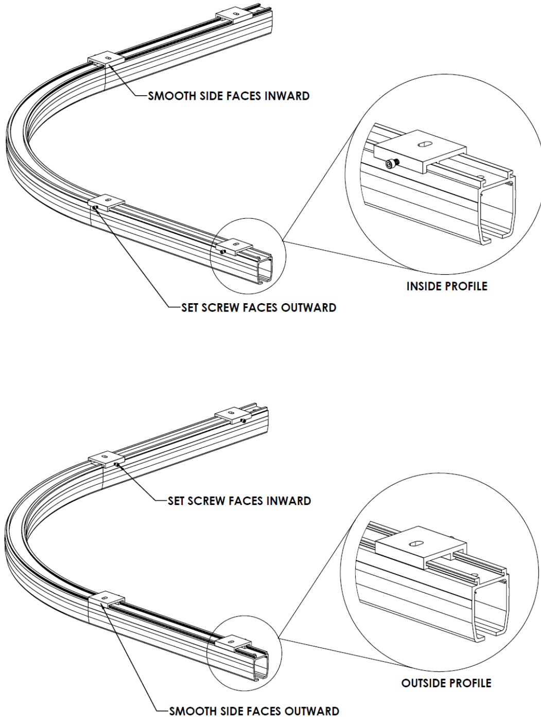
Figure 321: Ceiling Track Inside and Outside Curve Configurations (note placement of alignment tabs)
