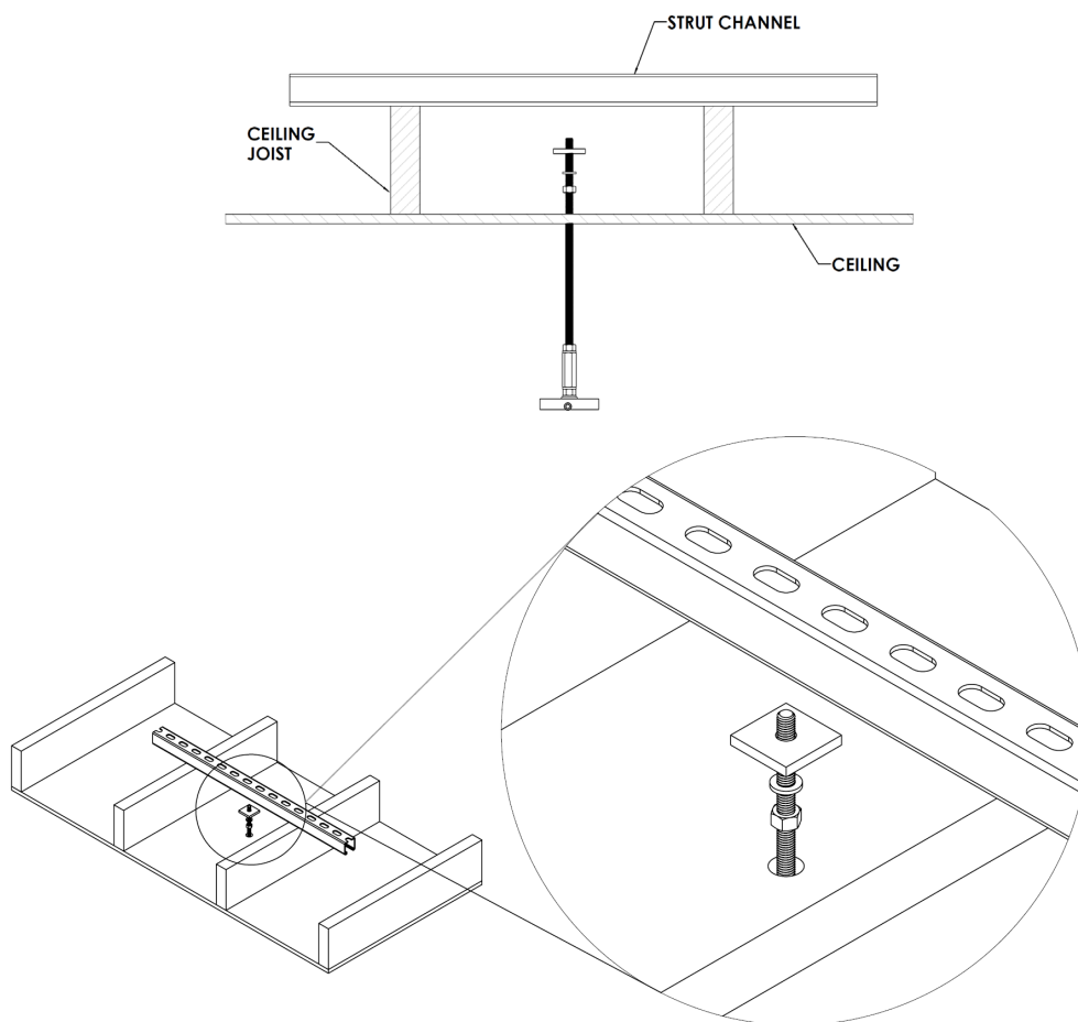
Figure 139: Hex Nut, Lock Washer, Square Washer Assembly
