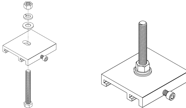
Figure 147: Flat Washer, Lock Washer, Hex Nut Assembly
