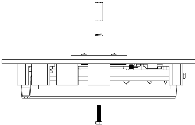
Figure 125: Attach Appropriate Mounting Hardware to the Turntable
