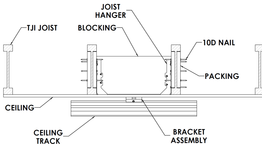
Figure 185: TJI Joist Packing Installation
