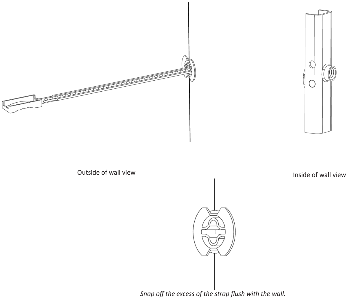
Figure 213: Installing the Flip Toggle
