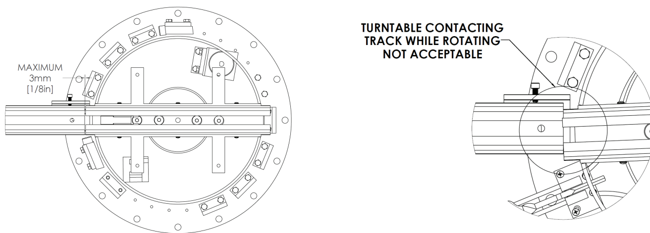
Figure 127: Gap Should be as Narrow as Possible Without Obstructing Proper Rotation
