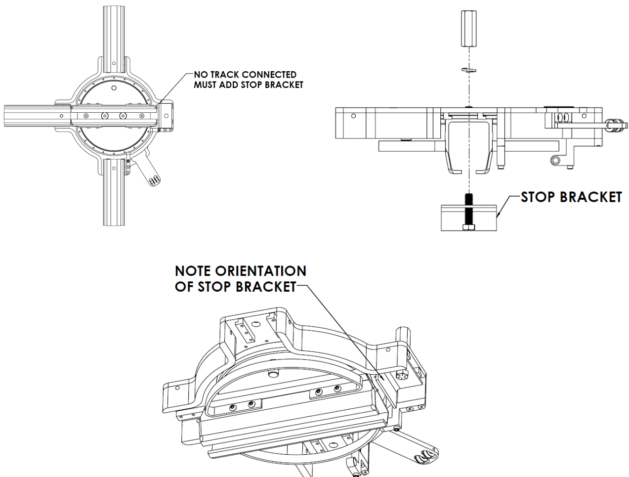
Figure 110: Install Stop Brackets at All Entry/Exit Points Where There is No Track
