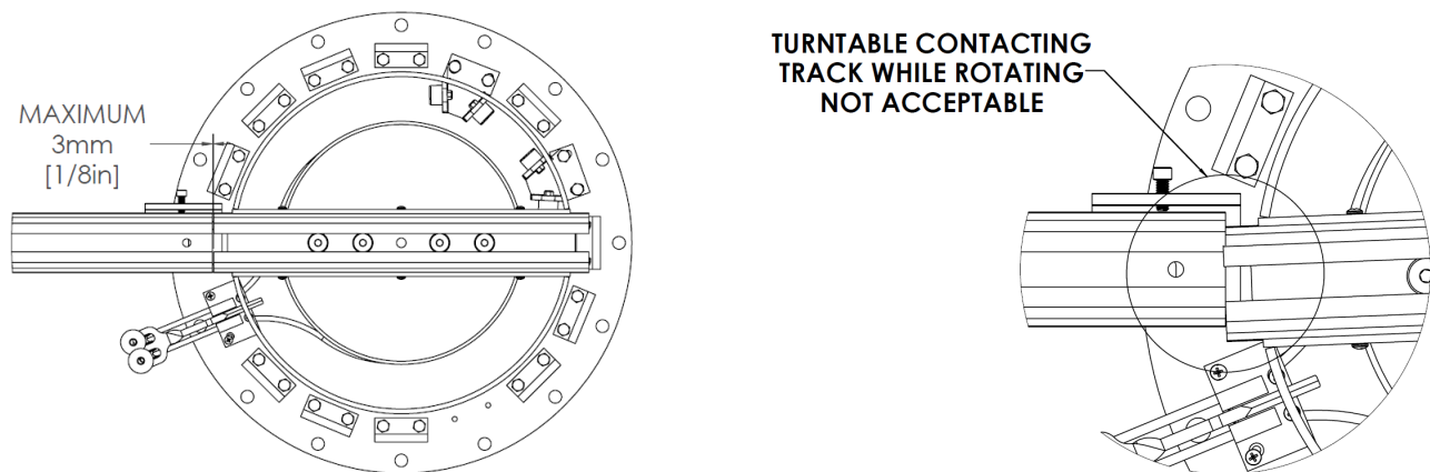
Figure 119: Gap Should be as Narrow as Possible Without Obstructing Proper Rotation
