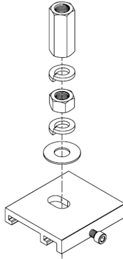
Figure 302: Flat Washer, Lock Washer, Hex Nut
