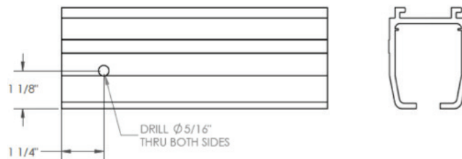
Figure 7: Clevis Pin Hole Location
