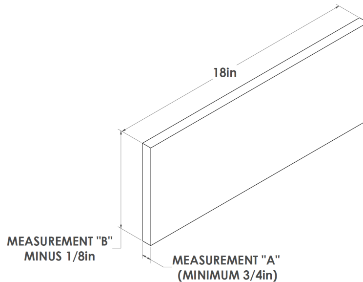
Figure 188: Cut Packing
