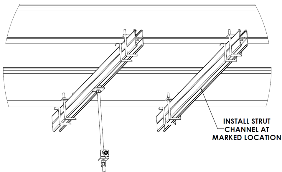
Figure 293: Install Additional Strut Channel
