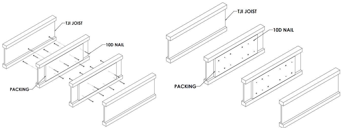
Figure 190: Nail Placement
