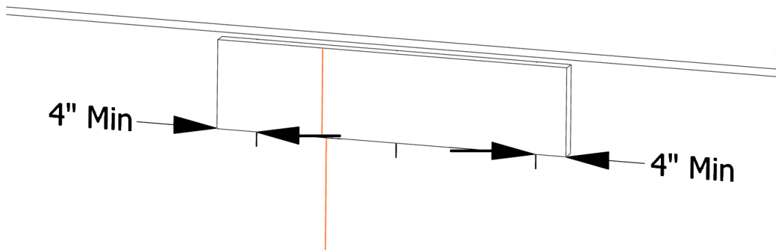
Figure 231: Minimum of 4" Past the Outer Joists on Both Sides
