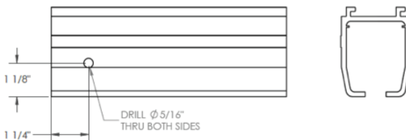
Figure 220: Clevis Pin Hole Location
