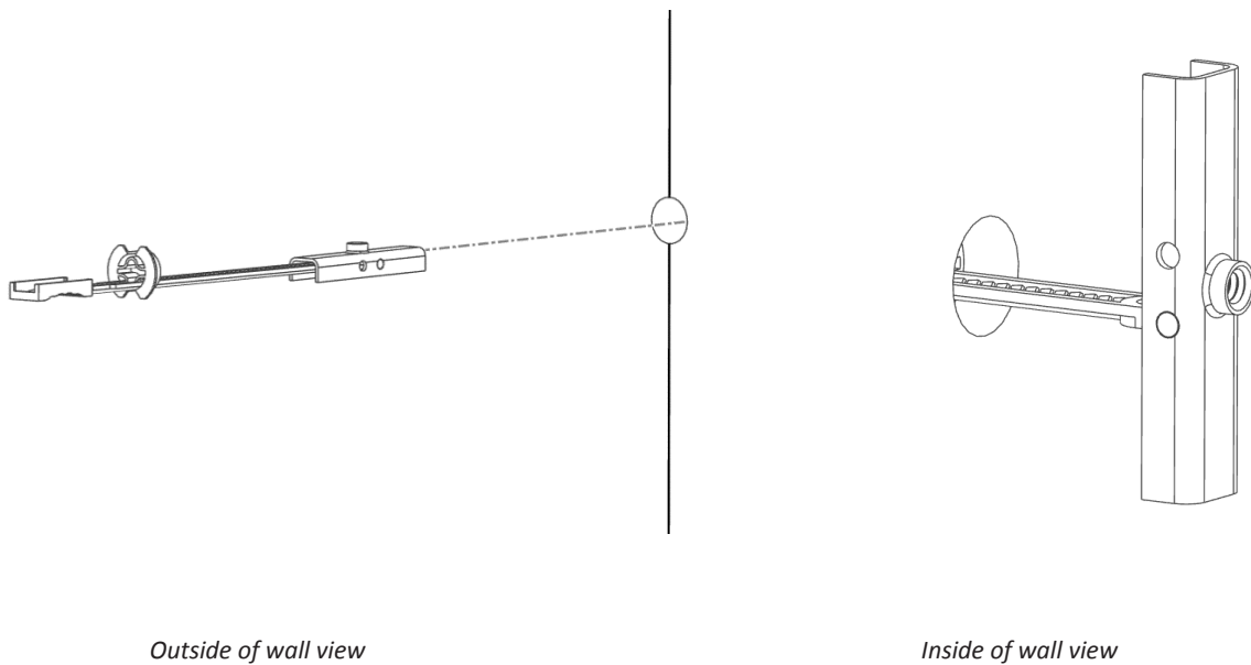
Figure 212: Flip Toggle
