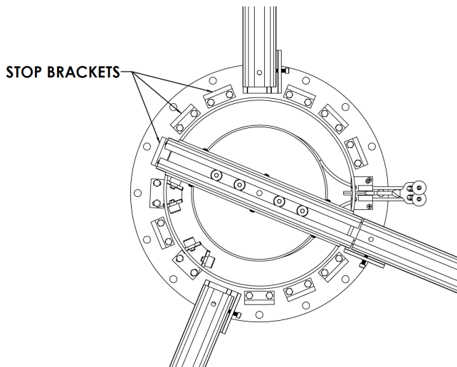
Figure 115: Stop Bracket Installation
