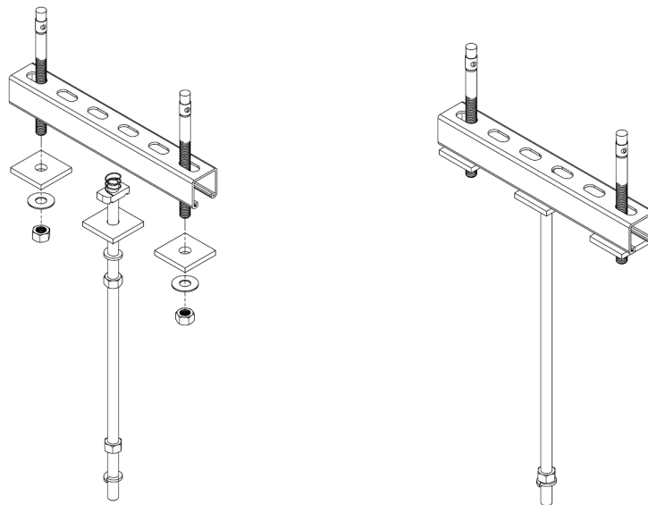
Figure 245: Vertical Attachment
