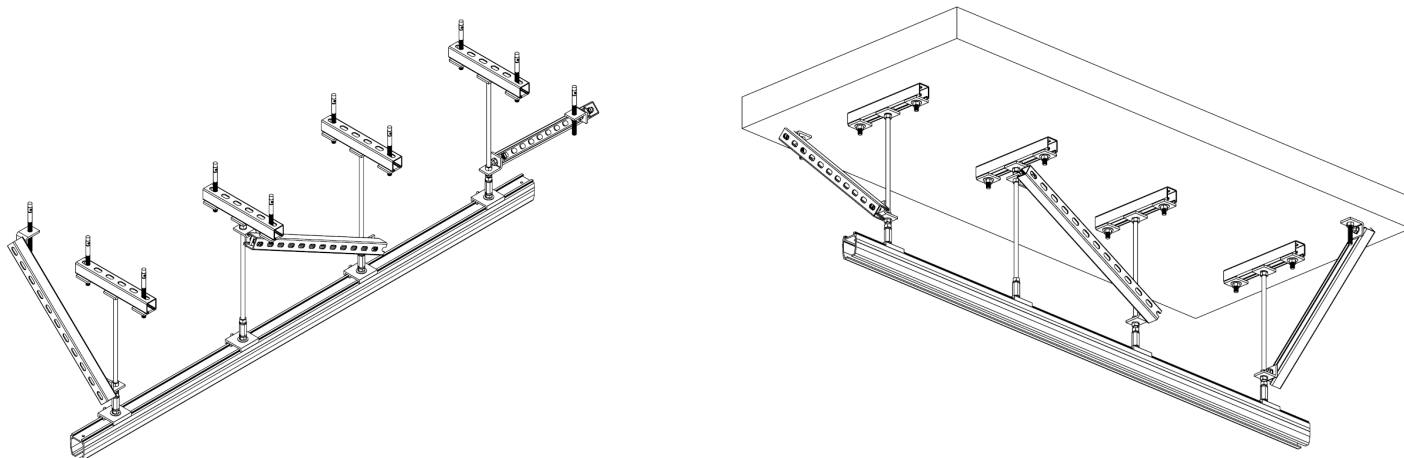
Figure 243: Concrete Installation
