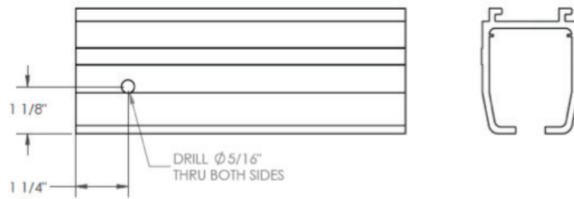
Figure 86: Clevis Pin Hole Location
