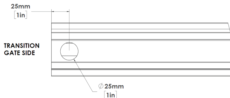
Figure 88: Traversing Track Hole
