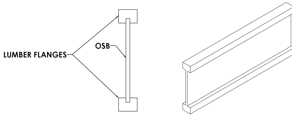
Figure 186: TJI Joist
