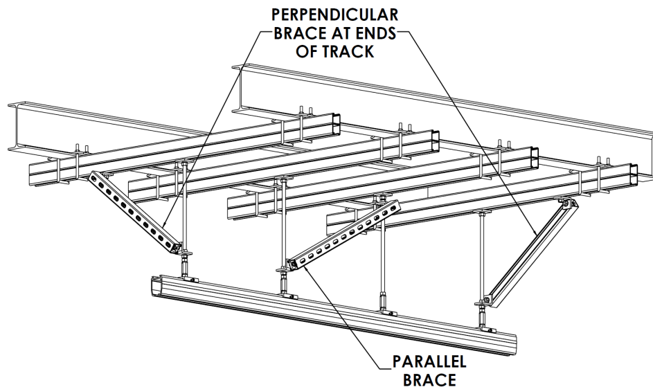
Figure 288: Lateral Bracing
