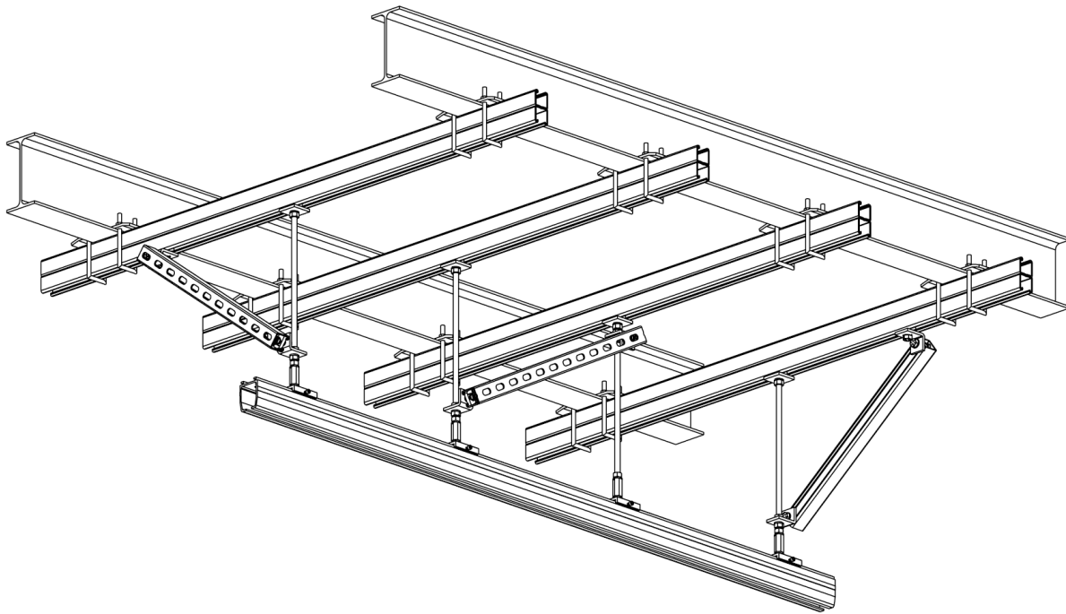
Figure 274: Structural Beam/Open Web Joist Installation
