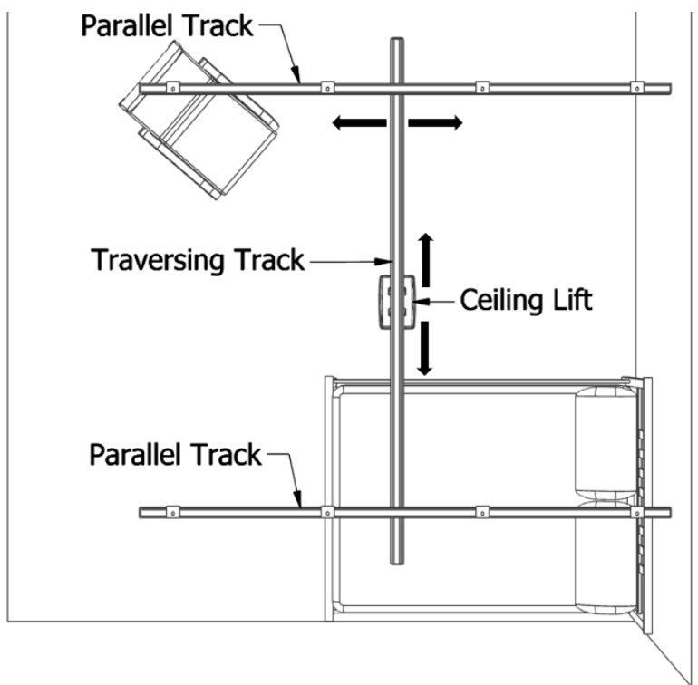
Figure 11: Typical Traverse Track (X/Y) System Set-Up
