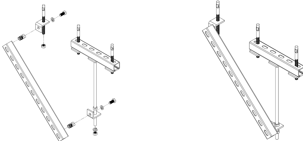
Figure 246: Lateral Bracing
