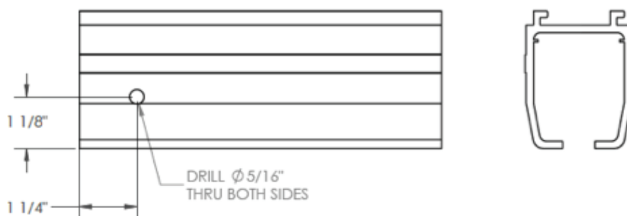
Figure 239: Clevis Pin Hole Location
