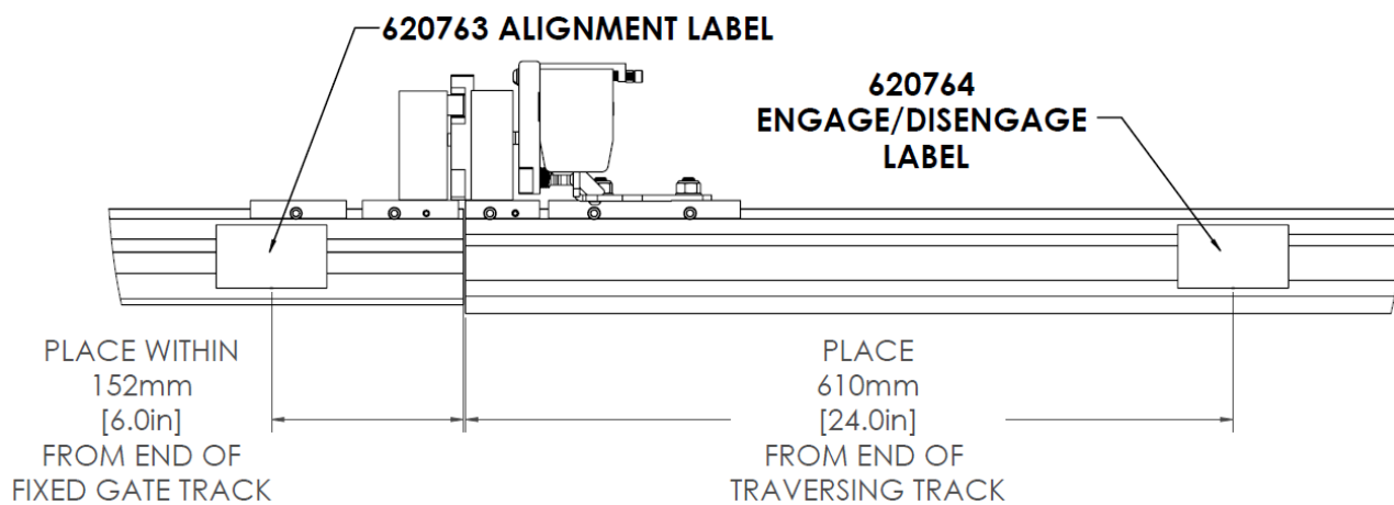
Figure 103: Install the Labels
