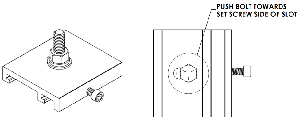
Figure 270: Tighten the Assembly
