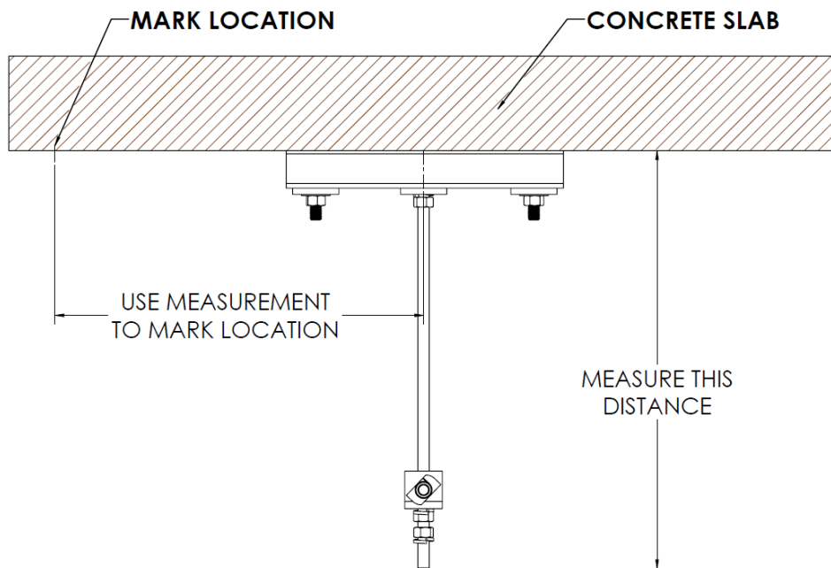
Figure 262: Mark the Location on the Concrete Slab
