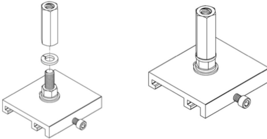
Figure 134: Lock Washer and Coupling Nut
