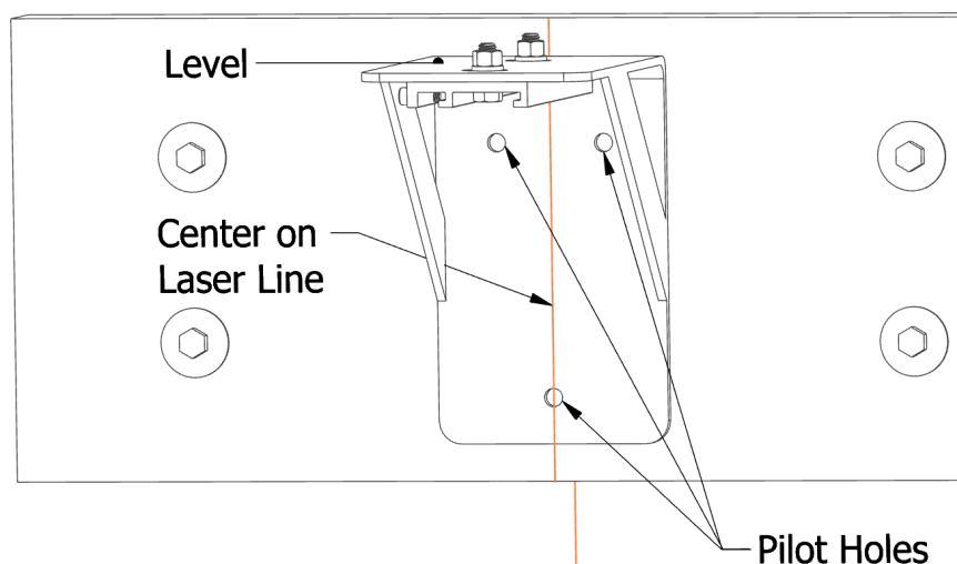
Figure 236: Wall Mount Bracket Assembly: Proper Orientation
