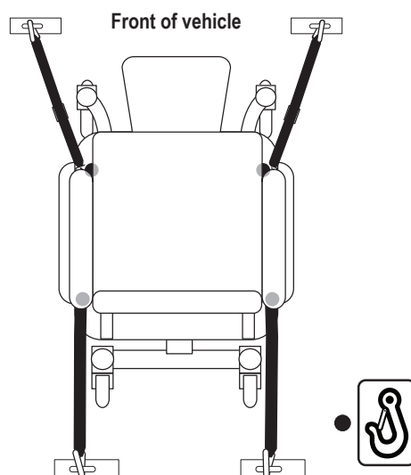
Figure 6. Unoccupied Transit System Securement Points
