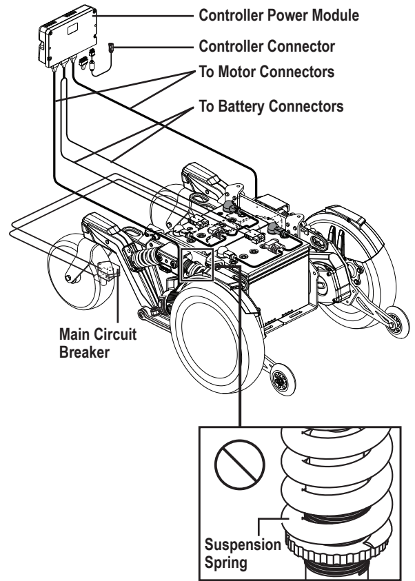
Figure 1. Quantum 4Front Series Electrical Components
